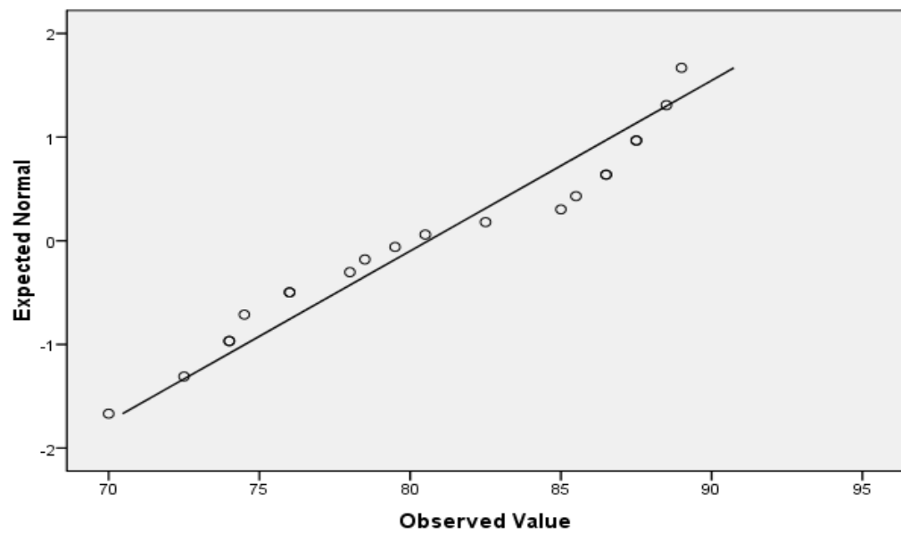
Normal Q-Q Plot of NILAI
